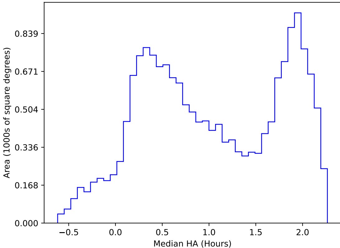
ddf_loaded_fl8_v3.4_10yrs WFD i band: Median HA
