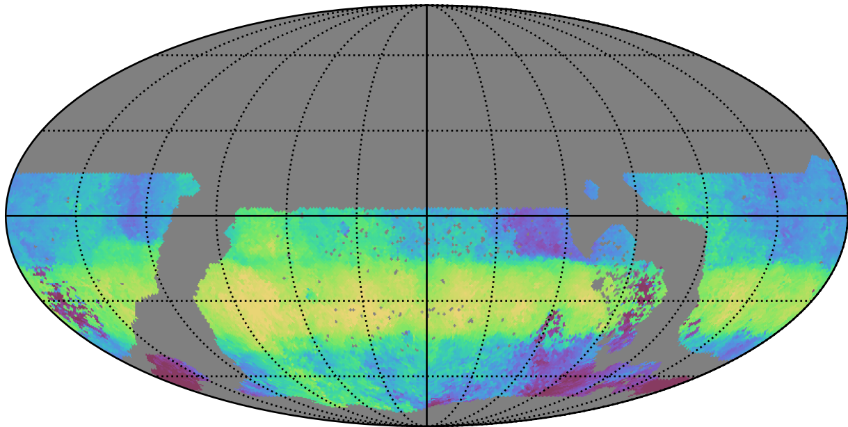
ddf_loaded_fl8_v3.4_10yrs WFD g band: Median HA
