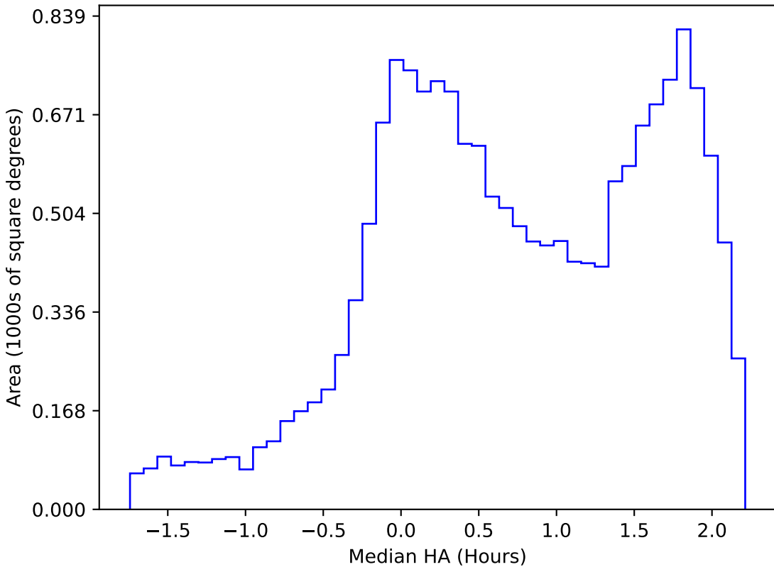
ddf_loaded_fl8_v3.4_10yrs WFD g band: Median HA
