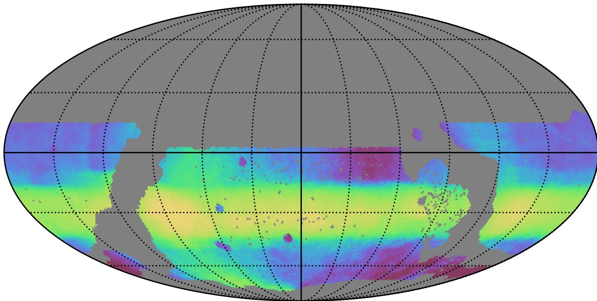
ddf_loaded_fl8_v3.4_10yrs WFD all bands: Median HA
