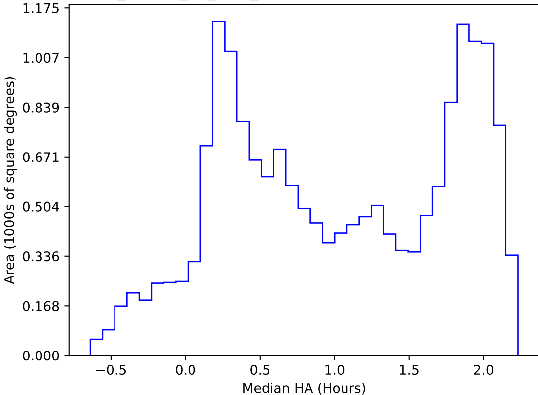
ddf_loaded_fl8_v3.4_10yrs WFD all bands: Median HA
