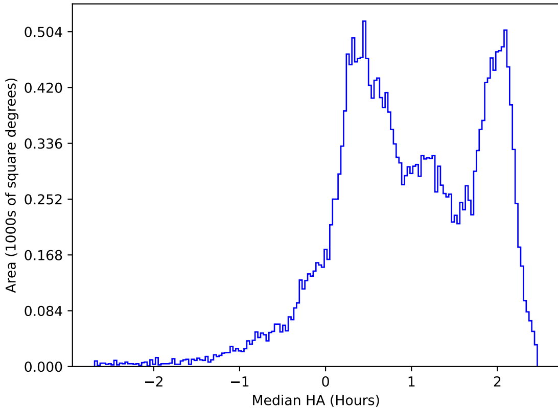
ddf_loaded_fl8_v3.4_10yrs All sky z band: Median HA
