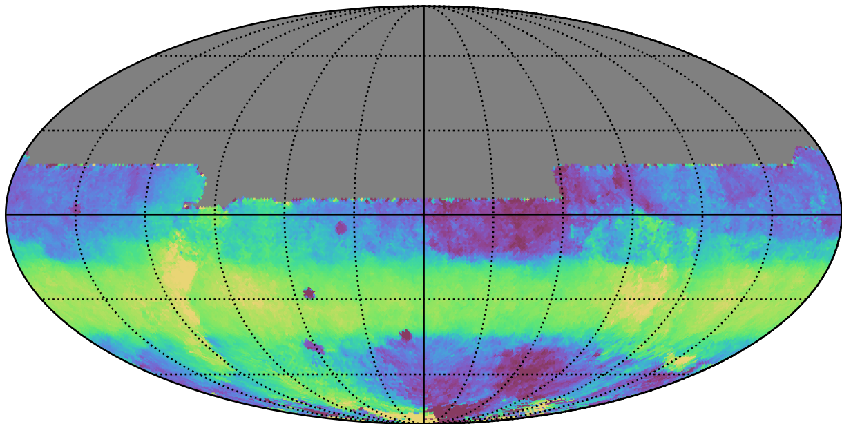
ddf_loaded_fl8_v3.4_10yrs All sky y band: Median HA
