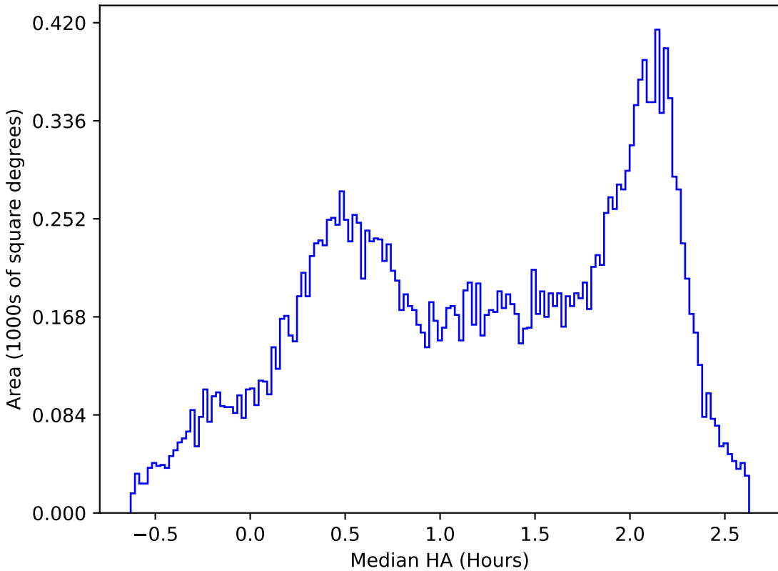
ddf_loaded_fl8_v3.4_10yrs All sky y band: Median HA
