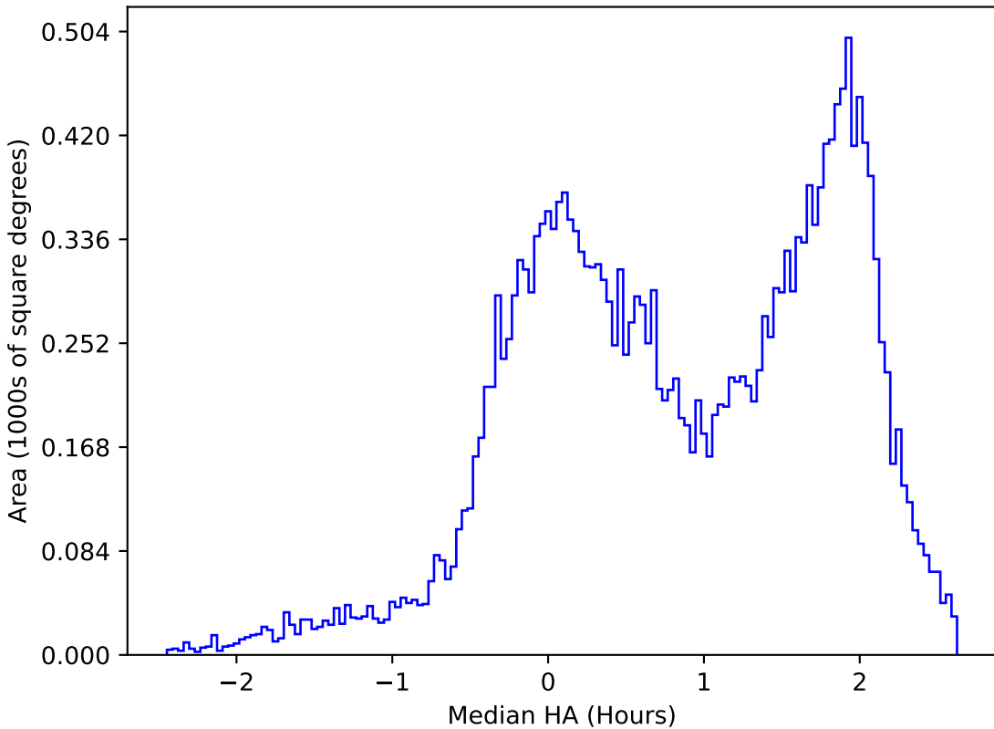
ddf_loaded_fl8_v3.4_10yrs All sky u band: Median HA
