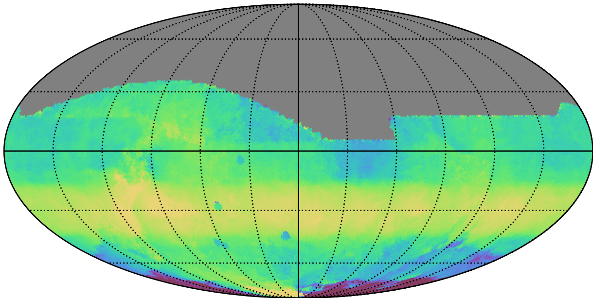
ddf_loaded_fl8_v3.4_10yrs All sky i band: Median HA
