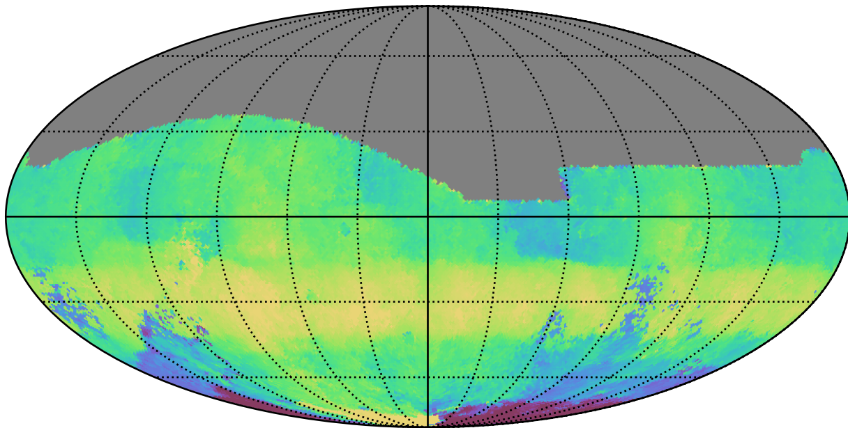
ddf_loaded_fl8_v3.4_10yrs All sky g band: Median HA
