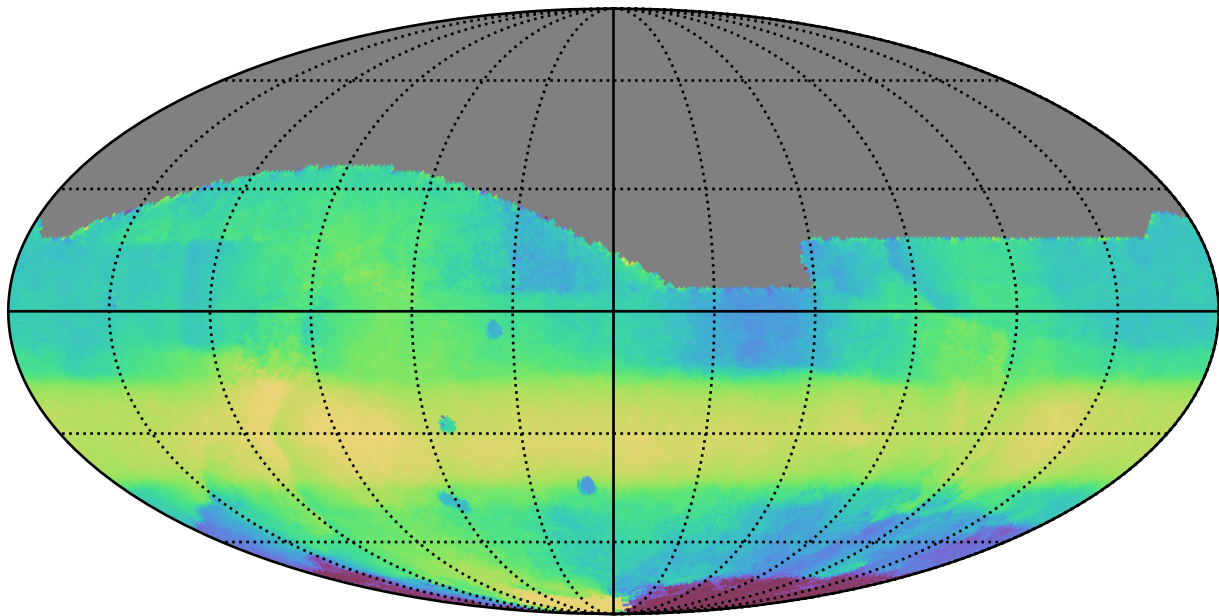
ddf_loaded_fl8_v3.4_10yrs All sky all bands: Median HA
