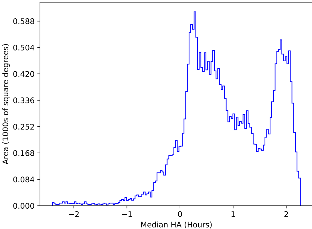
ddf_loaded_fl8_v3.4_10yrs All sky all bands: Median HA
