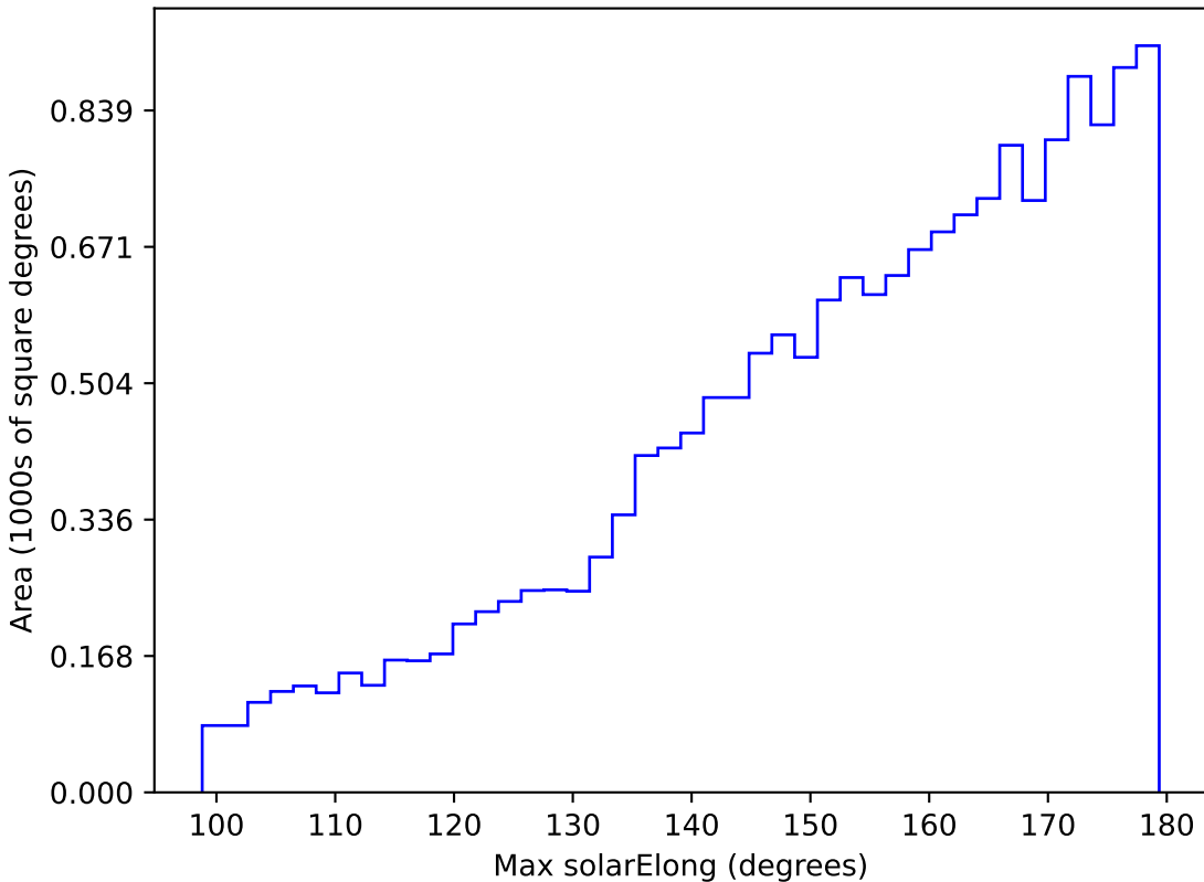
ddf_loaded_fl8_v3.4_10yrs WFD y band: Max solarElong
