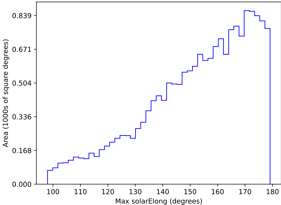
ddf_loaded_fl8_v3.4_10yrs WFD u band: Max solarElong
