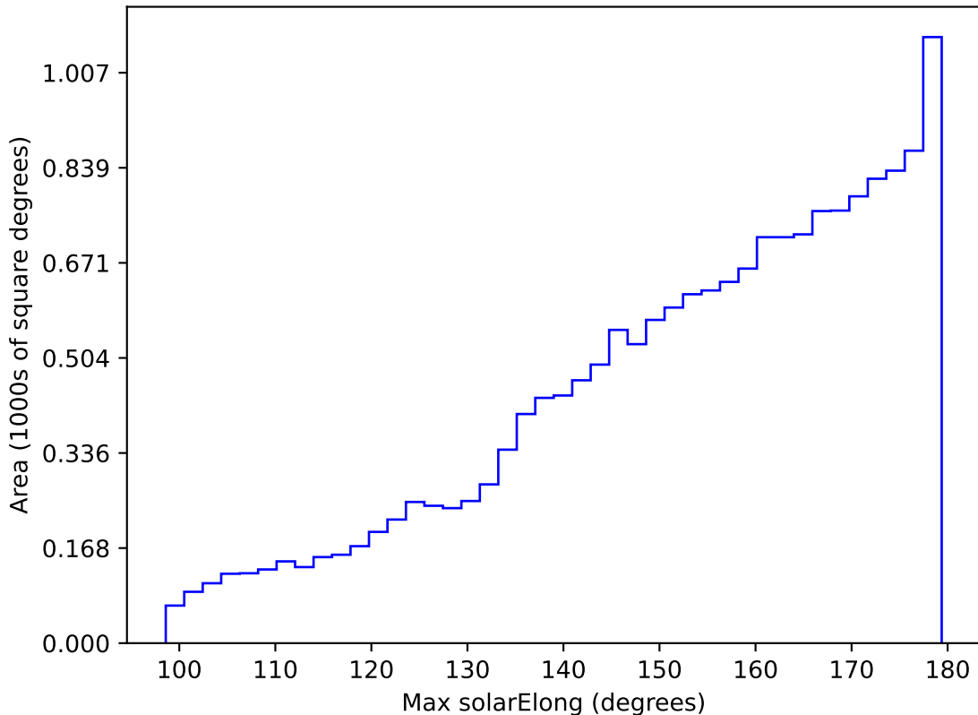
ddf_loaded_fl8_v3.4_10yrs WFD r band: Max solarElong
