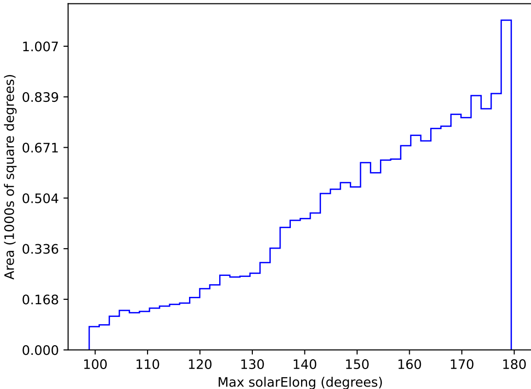
ddf_loaded_fl8_v3.4_10yrs WFD i band: Max solarElong
