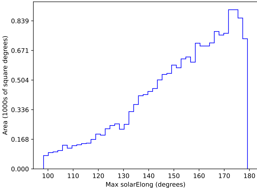
ddf_loaded_fl8_v3.4_10yrs WFD g band: Max solarElong
