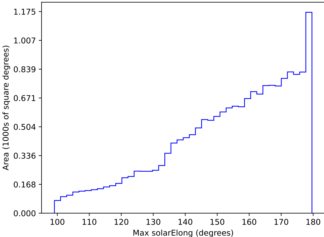
ddf_loaded_fl8_v3.4_10yrs WFD all bands: Max solarElong
