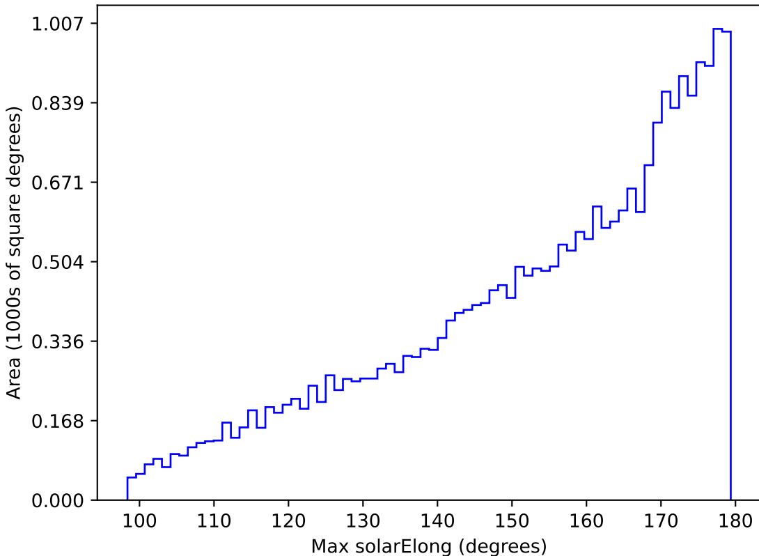
ddf_loaded_fl8_v3.4_10yrs All sky z band: Max solarElong
