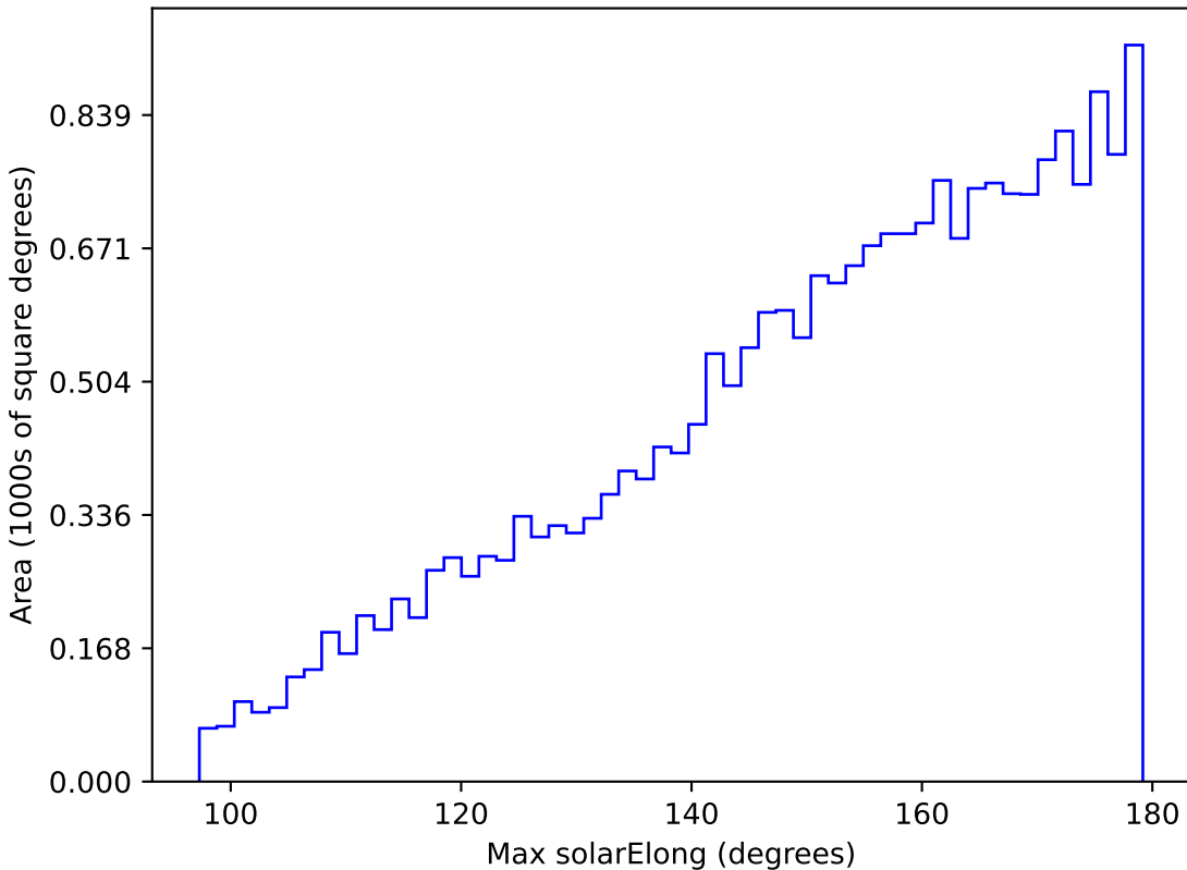
ddf_loaded_fl8_v3.4_10yrs All sky y band: Max solarElong
