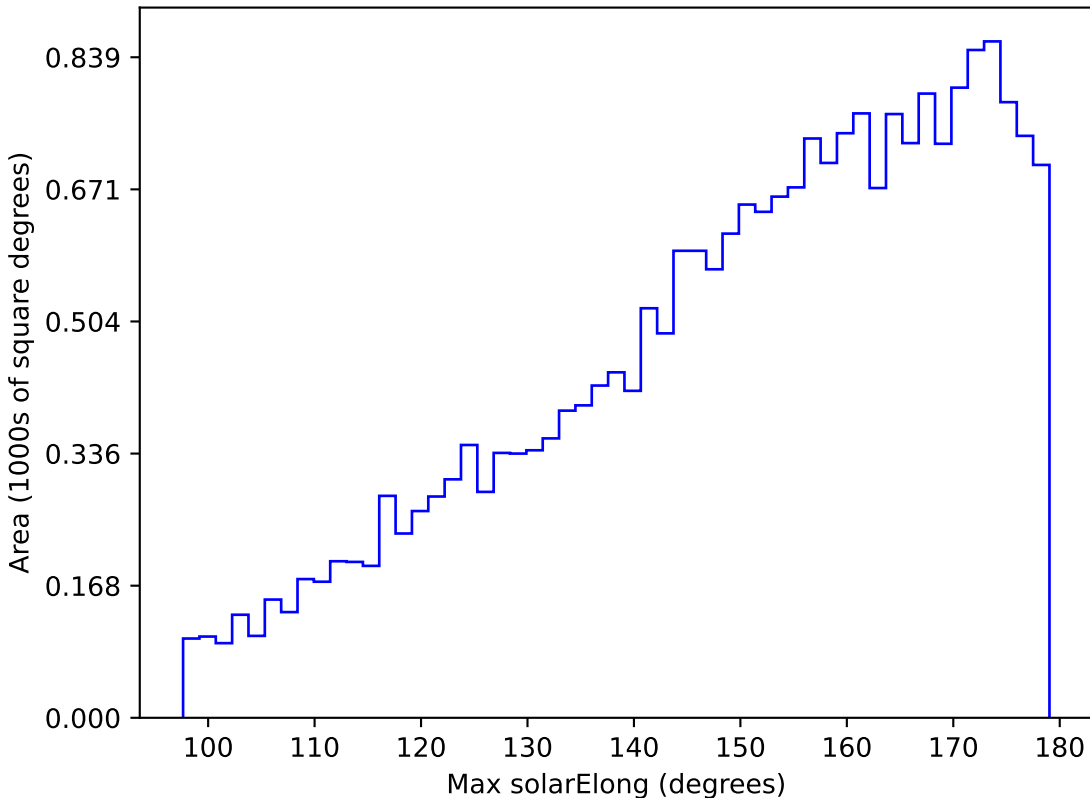
ddf_loaded_fl8_v3.4_10yrs All sky u band: Max solarElong
