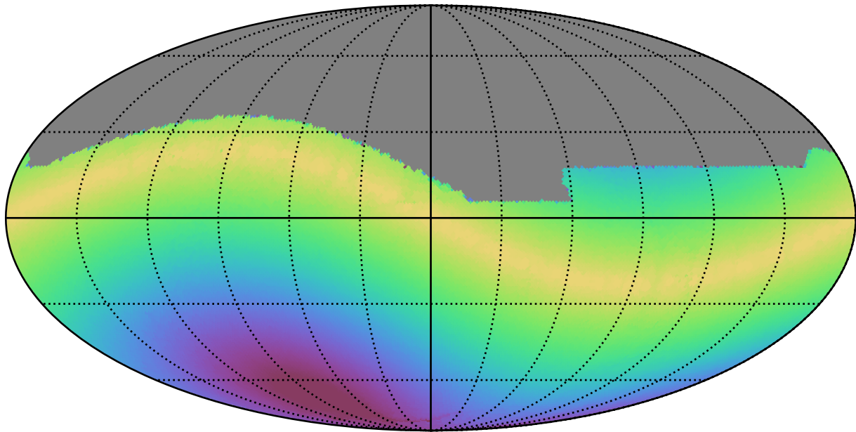
ddf_loaded_fl8_v3.4_10yrs All sky r band: Max solarElong
