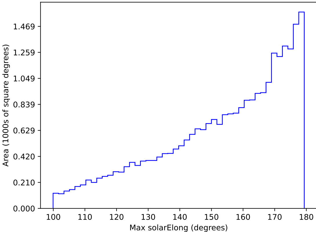
ddf_loaded_fl8_v3.4_10yrs All sky r band: Max solarElong
