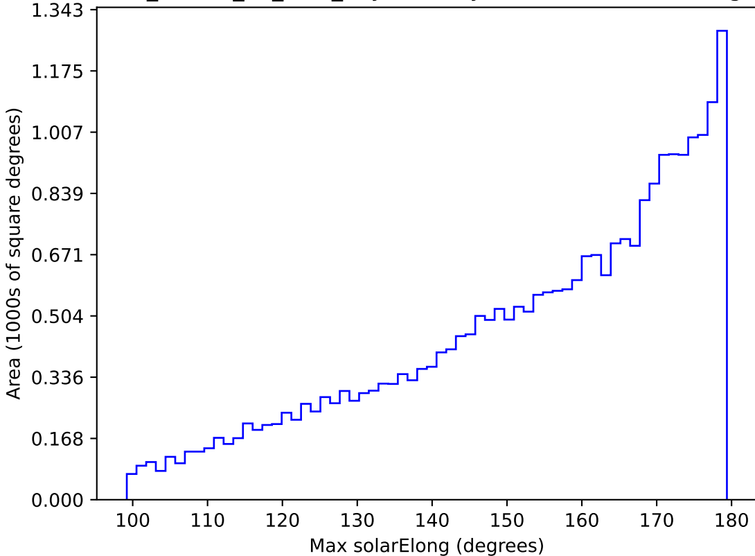
ddf_loaded_fl8_v3.4_10yrs All sky i band: Max solarElong
