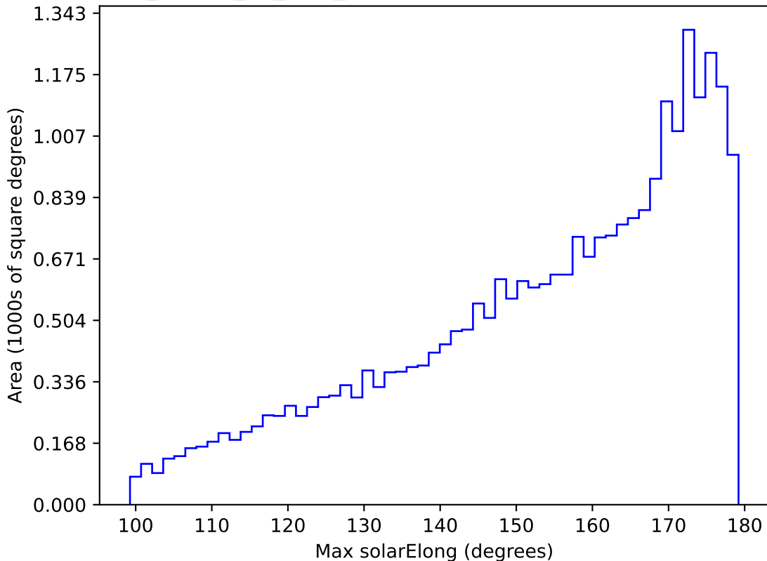
ddf_loaded_fl8_v3.4_10yrs All sky g band: Max solarElong
