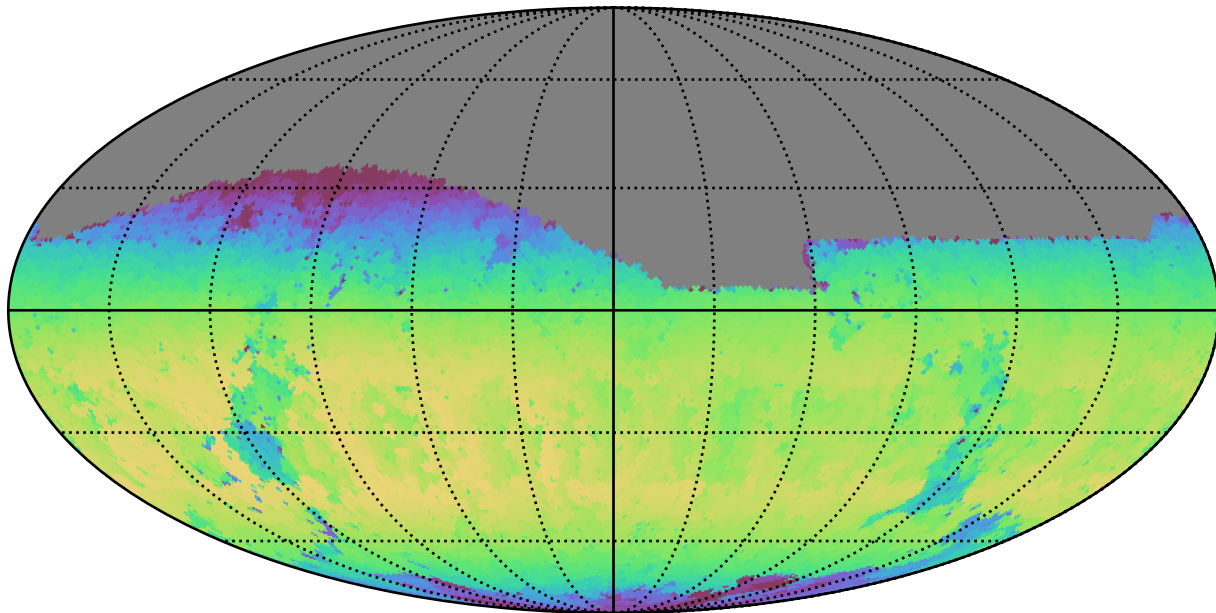
ddf_loaded_fl8_v3.4_10yrs Yr 1 z band: Max skyBrightness
