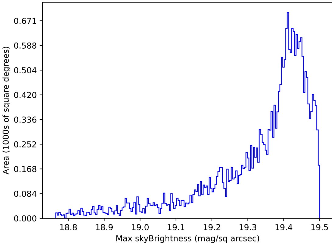
ddf_loaded_fl8_v3.4_10yrs Yr 1 z band: Max skyBrightness
