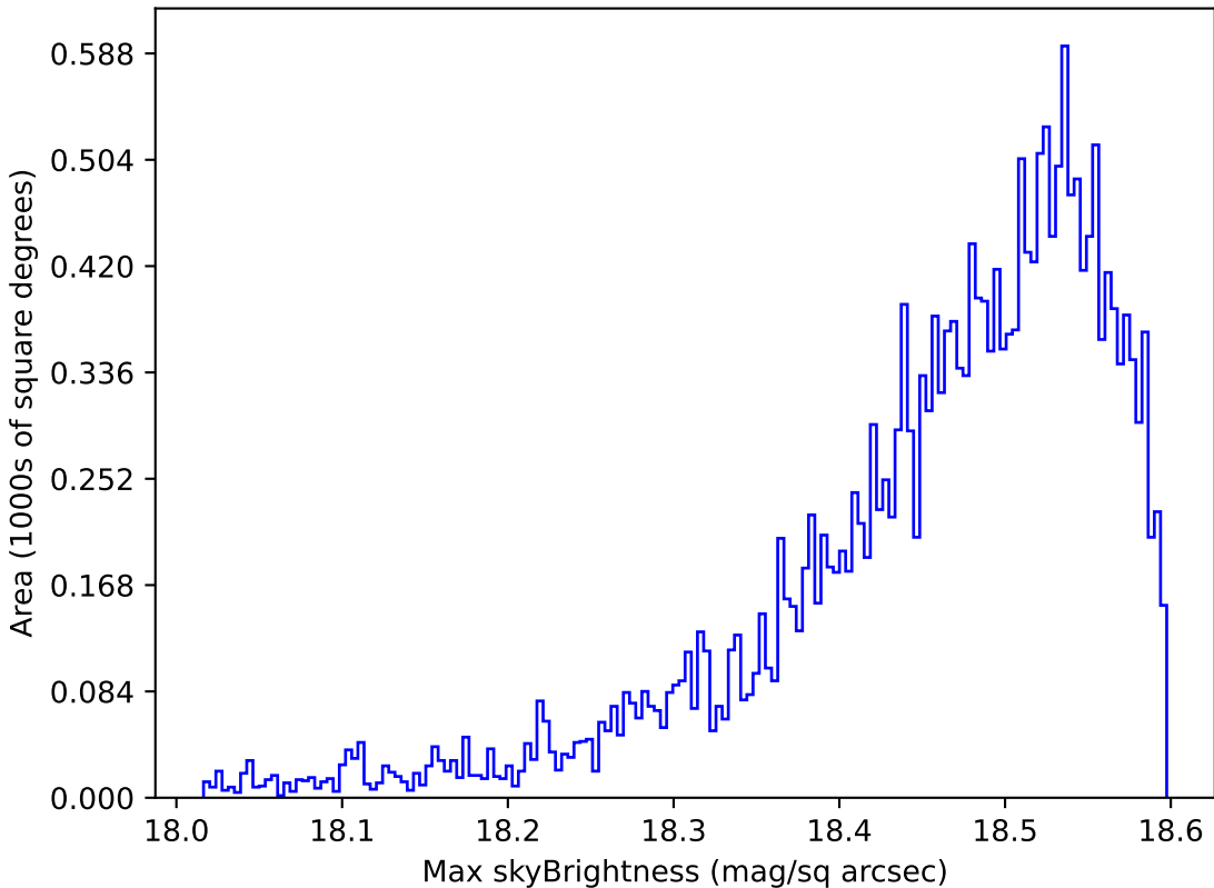
ddf_loaded_fl8_v3.4_10yrs Yr 1 y band: Max skyBrightness
