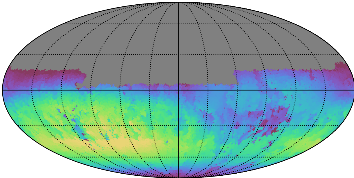
ddf_loaded_fl8_v3.4_10yrs Yr 1 u band: Max skyBrightness
