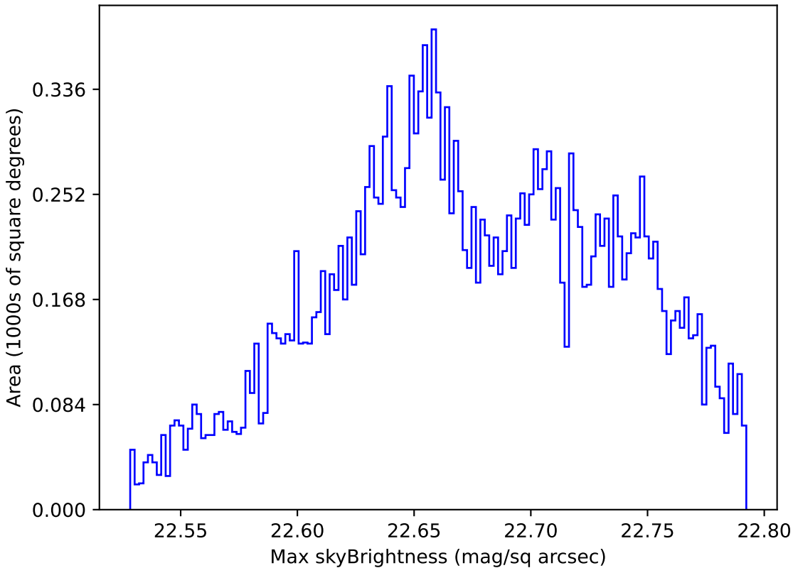
ddf_loaded_fl8_v3.4_10yrs Yr 1 u band: Max skyBrightness
