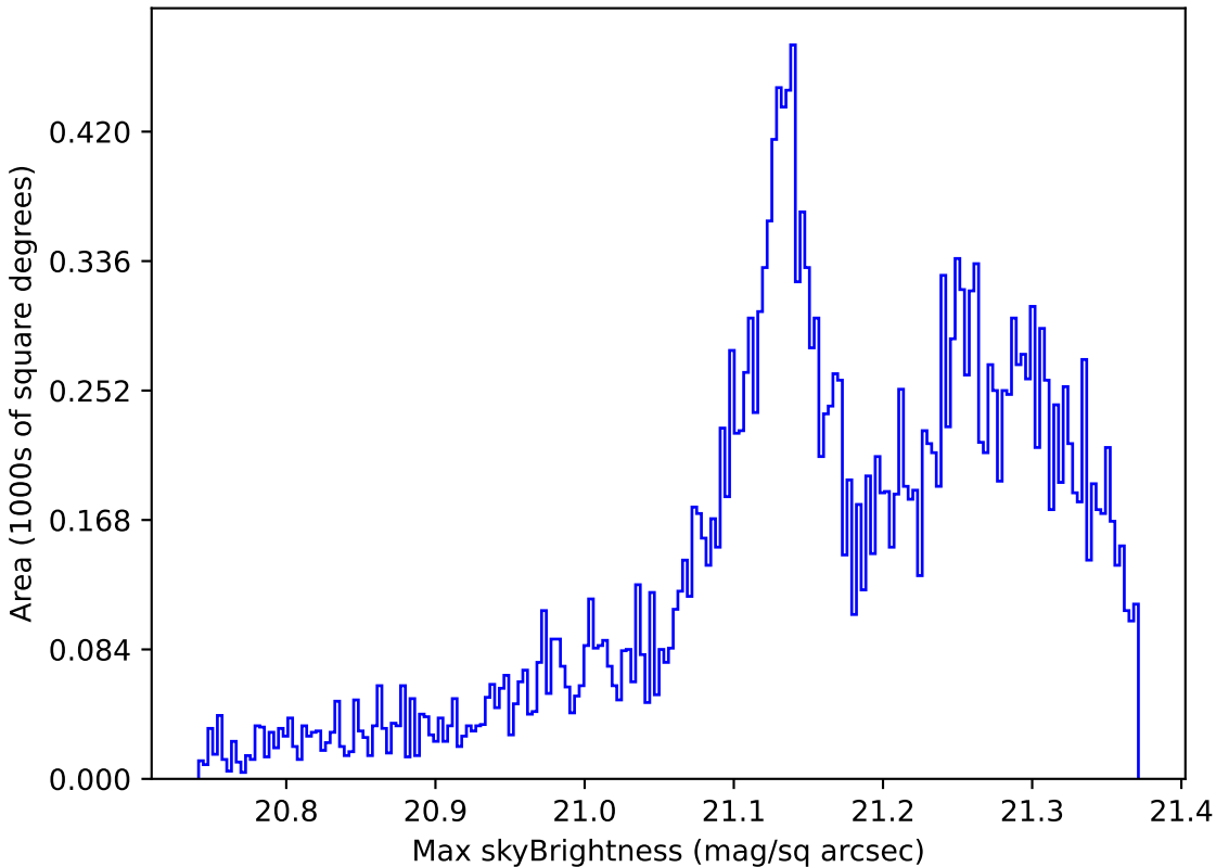
ddf_loaded_fl8_v3.4_10yrs Yr 1 r band: Max skyBrightness
