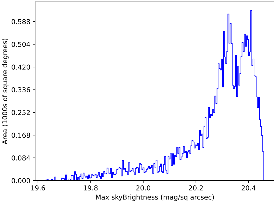
ddf_loaded_fl8_v3.4_10yrs Yr 1 i band: Max skyBrightness
