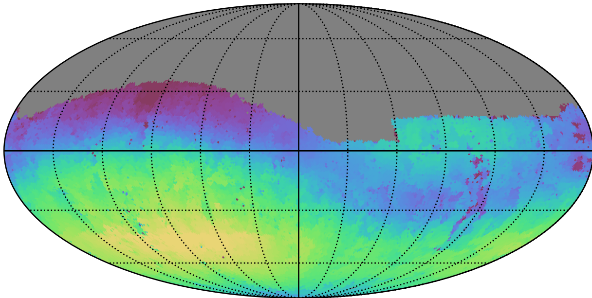
ddf_loaded_fl8_v3.4_10yrs Yr 1 g band: Max skyBrightness
