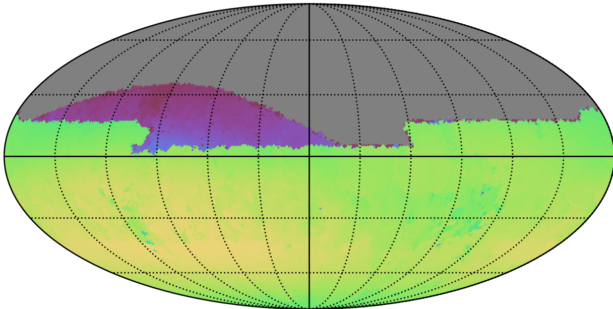
ddf_loaded_fl8_v3.4_10yrs Yr 1 all bands: Max skyBrightness
