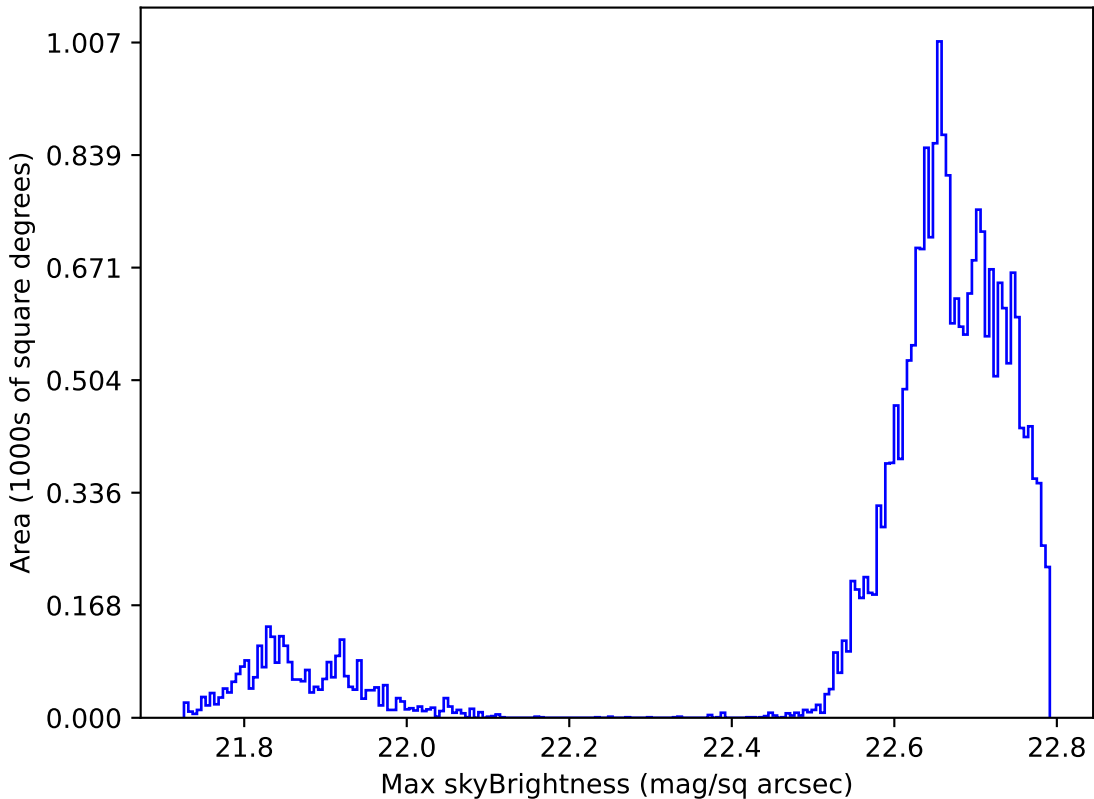
ddf_loaded_fl8_v3.4_10yrs Yr 1 all bands: Max skyBrightness
