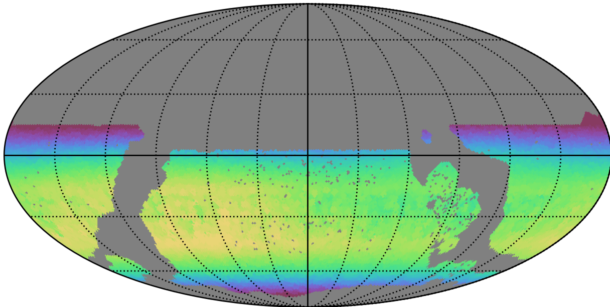
ddf_loaded_fl8_v3.4_10yrs WFD z band: Max skyBrightness
