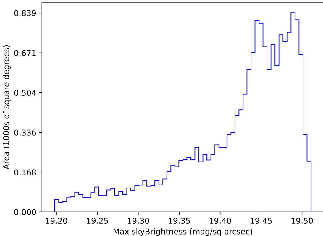
ddf_loaded_fl8_v3.4_10yrs WFD z band: Max skyBrightness
