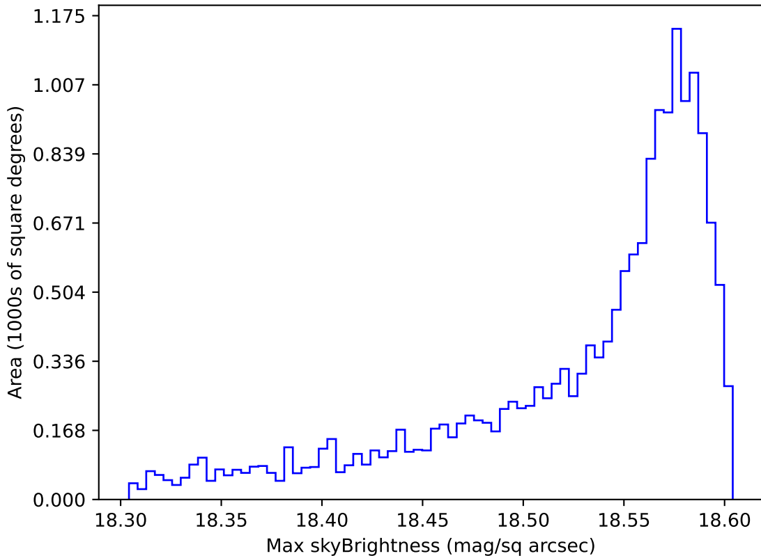
ddf_loaded_fl8_v3.4_10yrs WFD y band: Max skyBrightness
