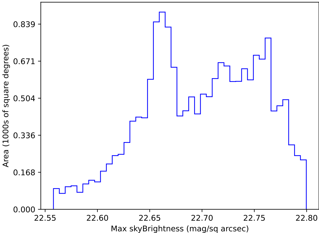
ddf_loaded_fl8_v3.4_10yrs WFD u band: Max skyBrightness
