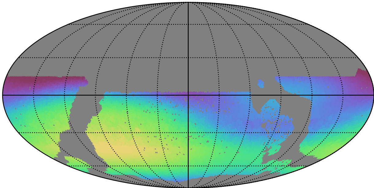
ddf_loaded_fl8_v3.4_10yrs WFD r band: Max skyBrightness
