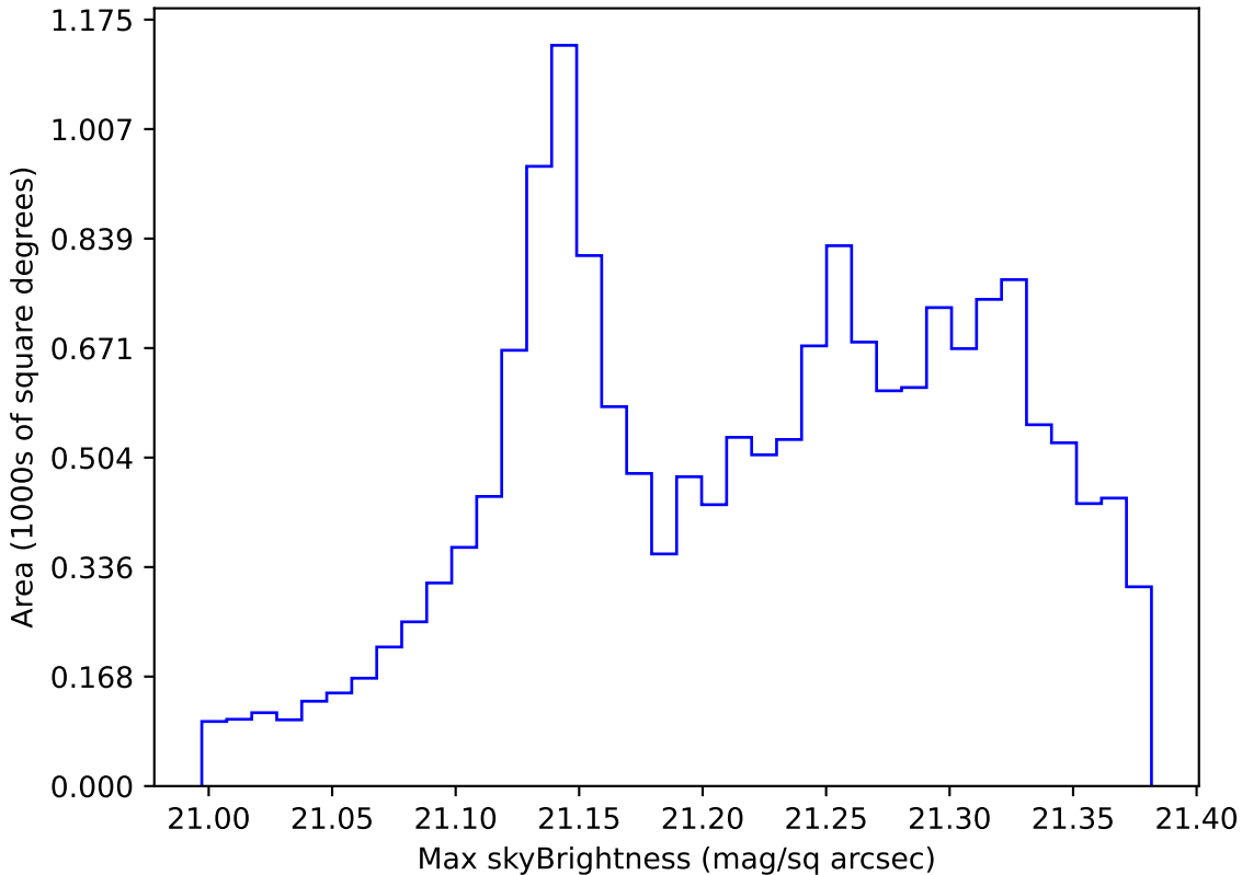
ddf_loaded_fl8_v3.4_10yrs WFD r band: Max skyBrightness
