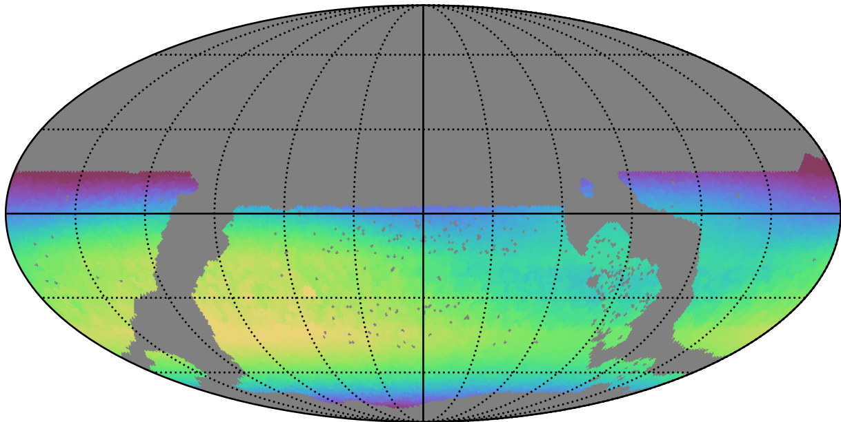
ddf_loaded_fl8_v3.4_10yrs WFD i band: Max skyBrightness
