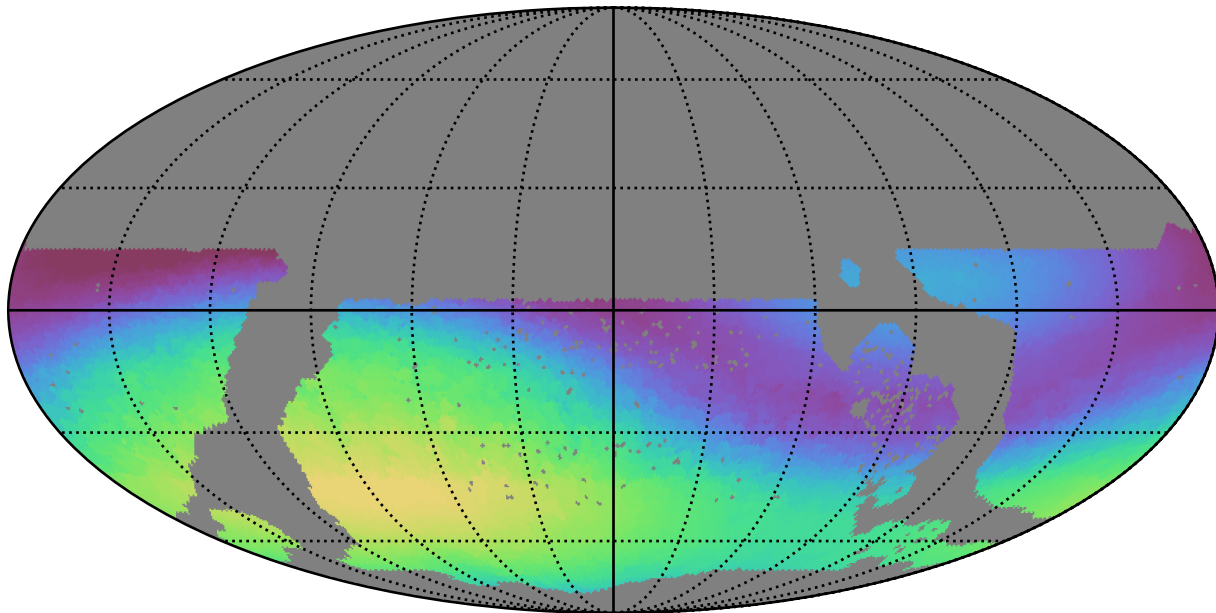
ddf_loaded_fl8_v3.4_10yrs WFD g band: Max skyBrightness
