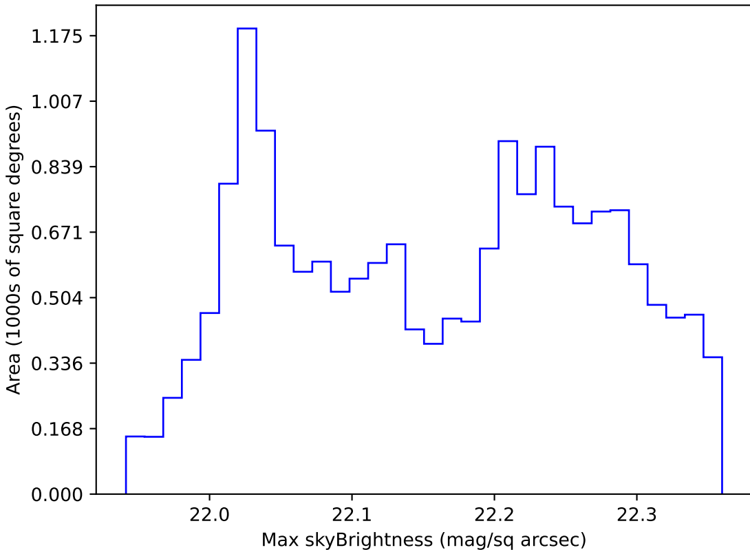
ddf_loaded_fl8_v3.4_10yrs WFD g band: Max skyBrightness
