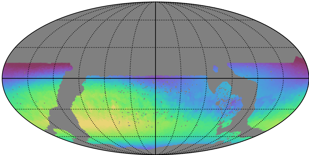
ddf_loaded_fl8_v3.4_10yrs WFD all bands: Max skyBrightness
