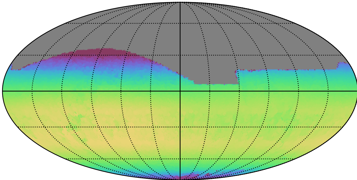
ddf_loaded_fl8_v3.4_10yrs All sky z band: Max skyBrightness
