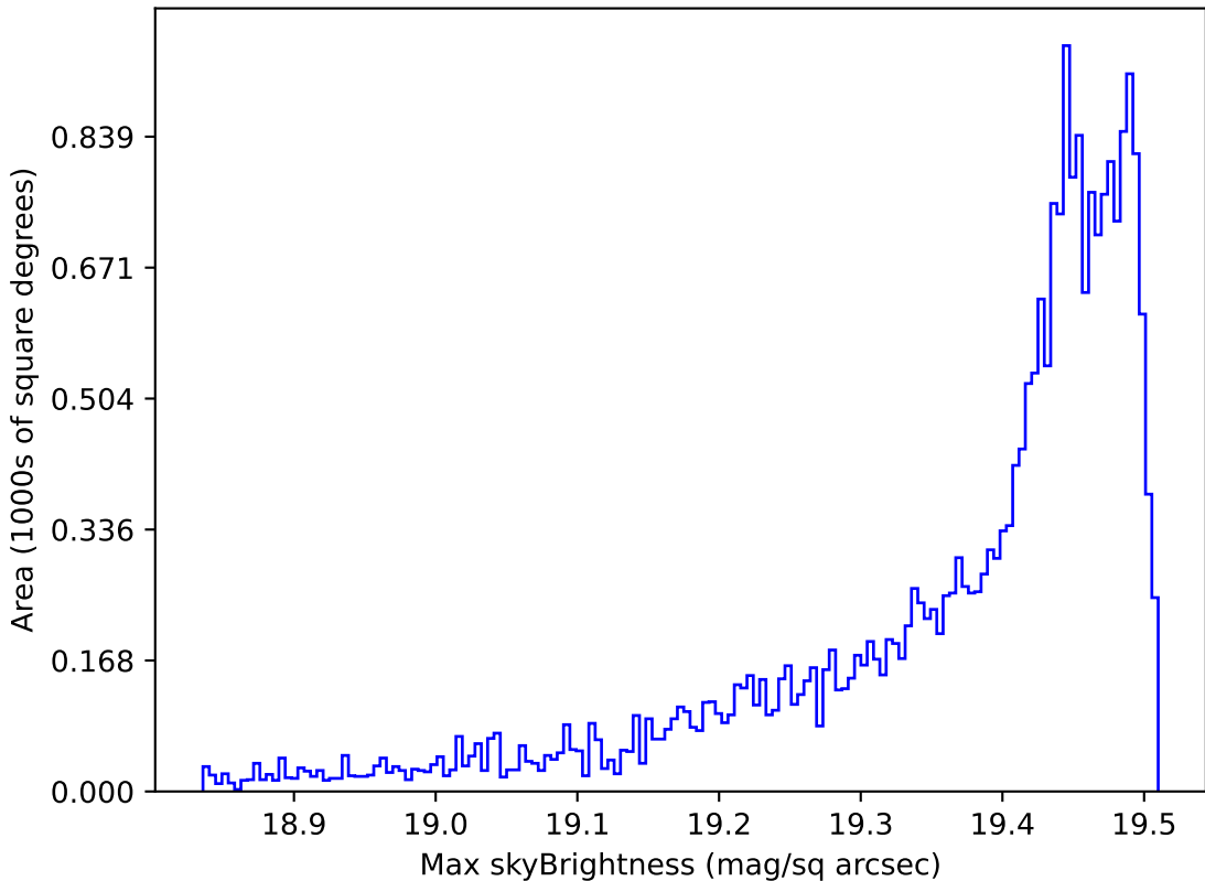
ddf_loaded_fl8_v3.4_10yrs All sky z band: Max skyBrightness
