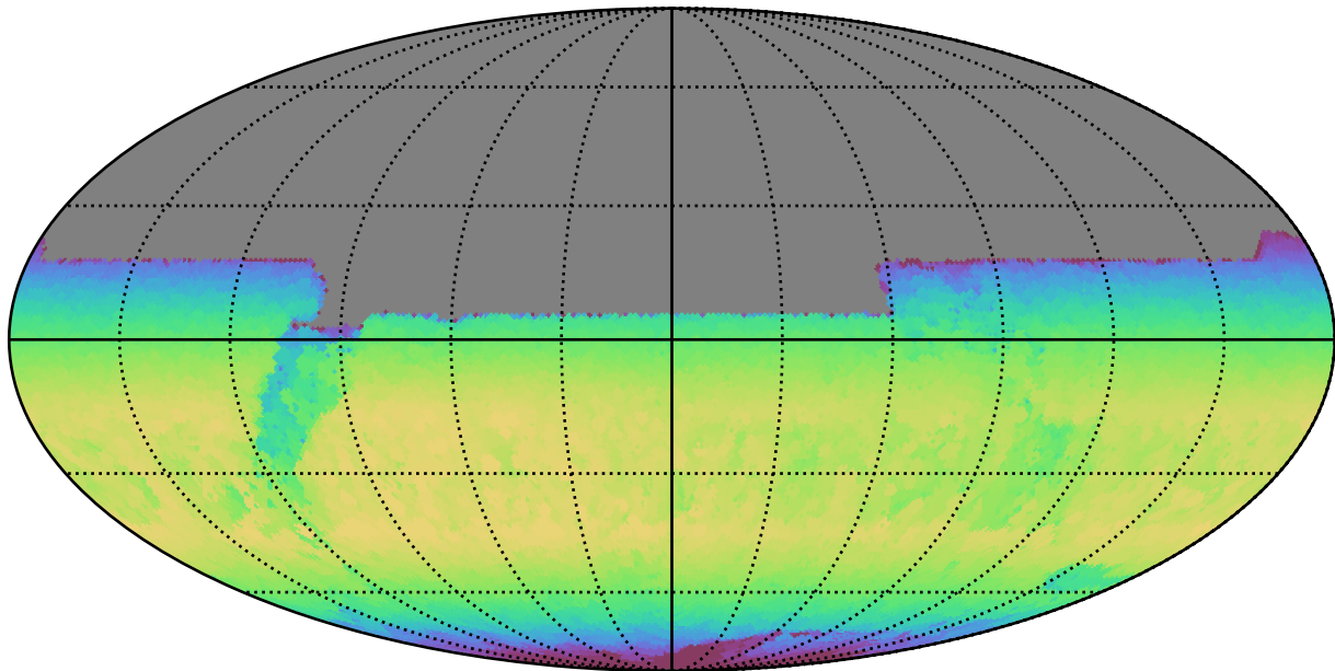
ddf_loaded_fl8_v3.4_10yrs All sky y band: Max skyBrightness
