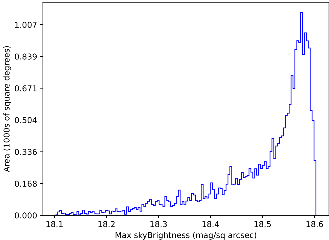
ddf_loaded_fl8_v3.4_10yrs All sky y band: Max skyBrightness
